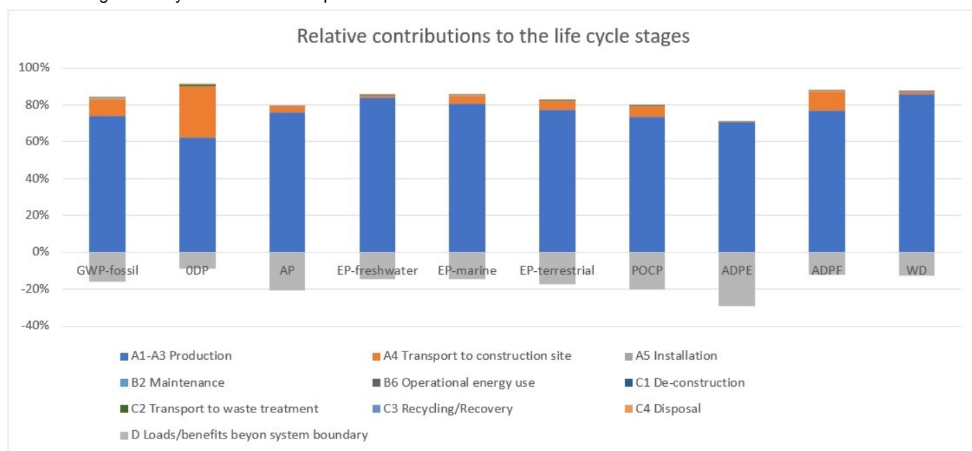
Figure 1: Environmental impacts of padlocks along its life cycle
